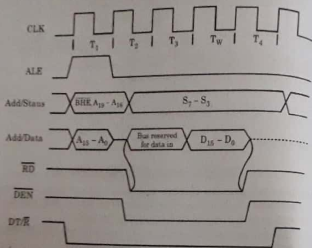
Fig. 3.9.1. Read cycle.
