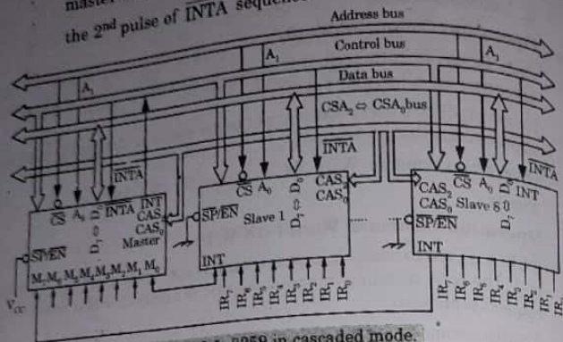
Fig. 5.20.1. 8259 in cascaded mode.
