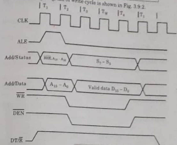
Fig. 3.9.2. Write cycle.
