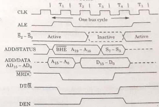
Fig. 3.11.1. Memory read timing in maximum mode.
