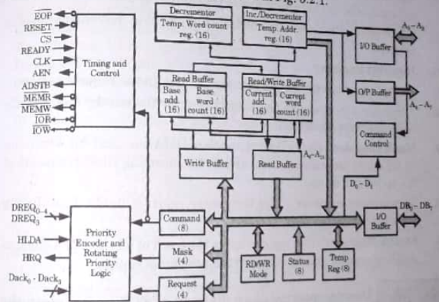
Fig. 5.2.1. Block diagram of 8237.
