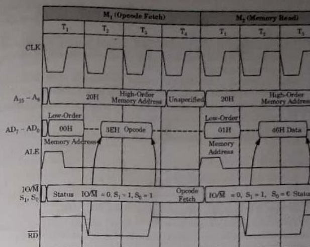
Fig. 2.9.1. 8085 Timing for execution of the instruction MVI A, 46H.
