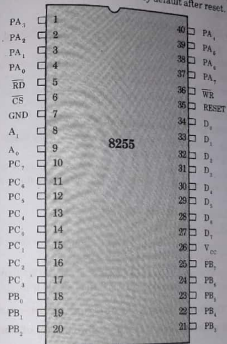
Fig. 5.6.1. 8255 pin configuration.
