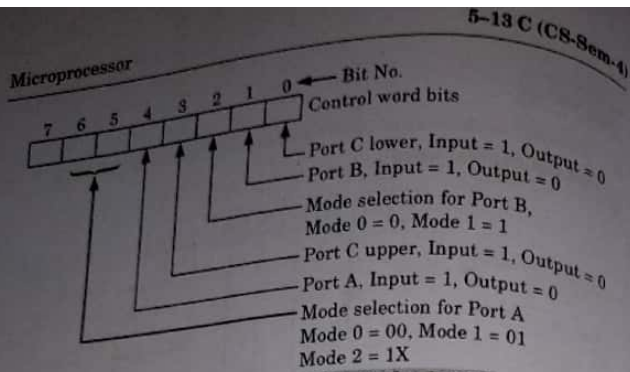
Fig. 5.9.1. Control word bits for Intel 8255.
