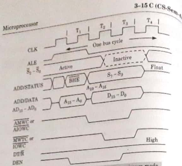
Fig. 3.11.2. Memory write timing in maximum mode.
