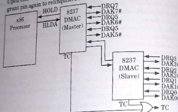
Fig. 5.4.1. Interfacing 8257/37 with 8086.
