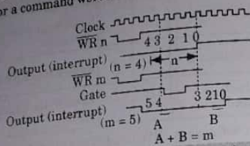
Fig. 5.14.1. Mode 0 : Interrupt on terminal count.
