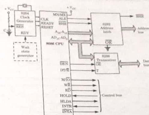
Fig. 3.8.1. Minimum mode 8086 system.
