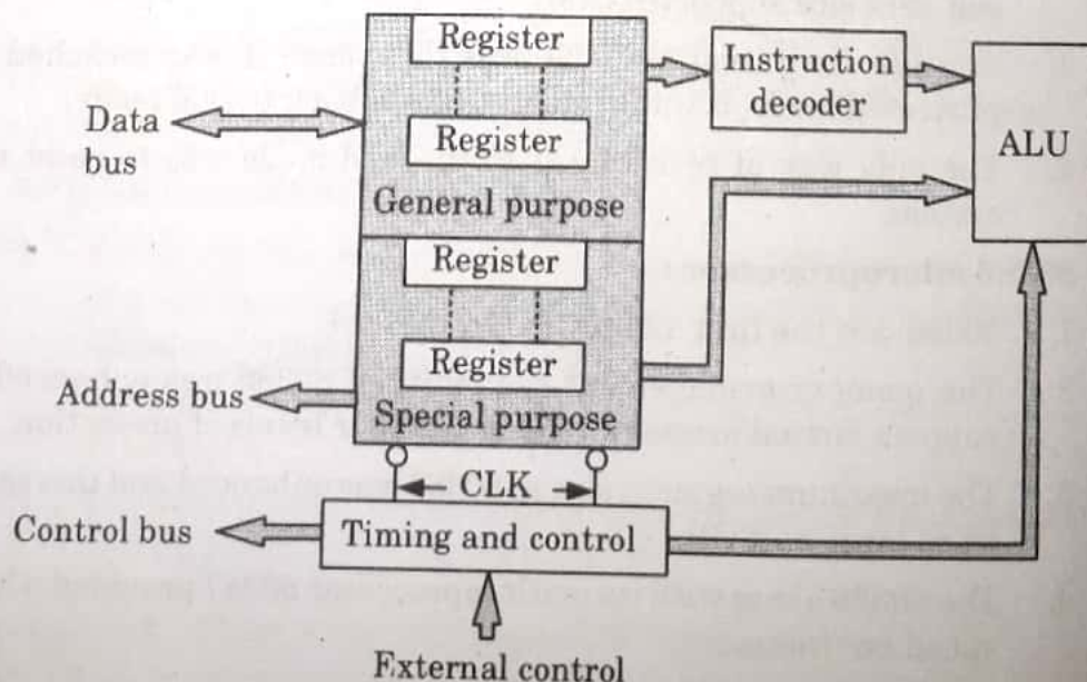
Fig. 1.4.1. General architecture of a microprocessor.
