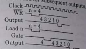
Fig. 5.14.5. Software triggered strobe.
