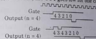
Fig. 5.14.6. Hardware triggered strobe.
