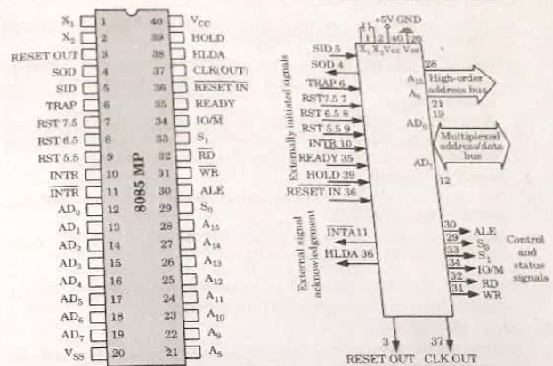
Fig. 2.2.1. Pin configuration and functional pin diagram.
