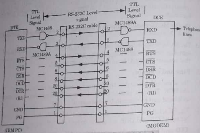
Fig. 5.24.1. The RS-232C pins and signals.
