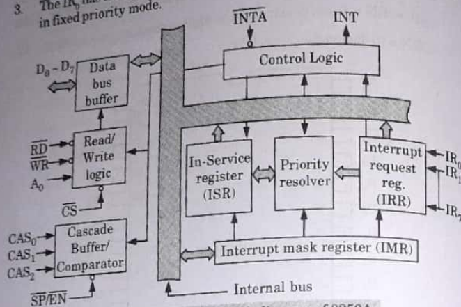
Fig. 5.17.1. Functional block diagram of 8259A.
