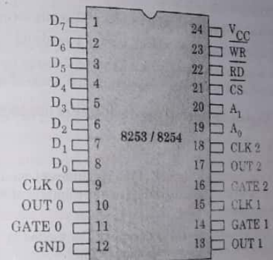
Fig. 5.12.1. Pin Configuration.
