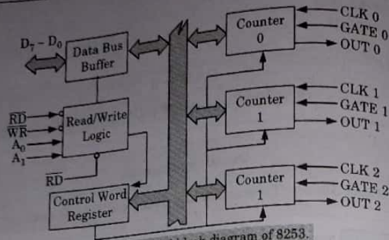
Fig. 5.11.1. Internal block diagram of 8253.
