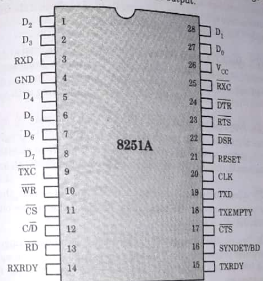
Fig. 5.23.1. 8251A pin configuration.
