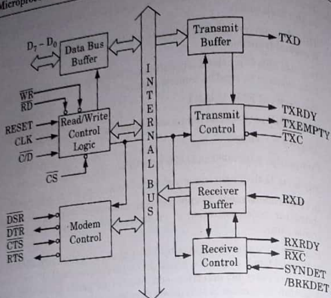
Fig. 5.22.1. 8251A Internal architecture.
